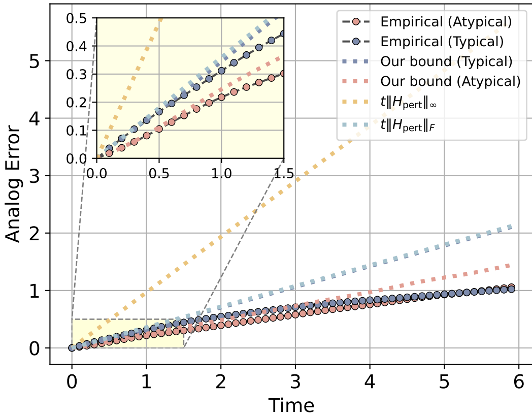
TFIM, long-time evolution with disorder
